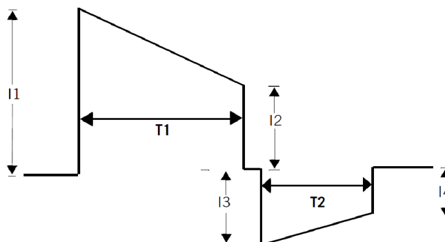
Biphasic Waveform
