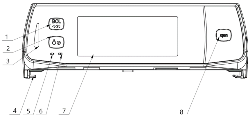
Figure 6-1-1 Front view
