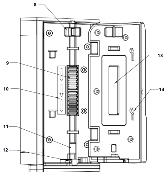
Figure 6-1-2 Side view
