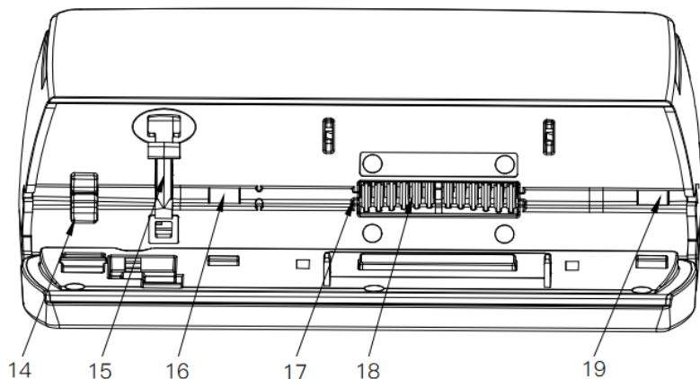
Figure 6-1-5 Pump door open diagram
